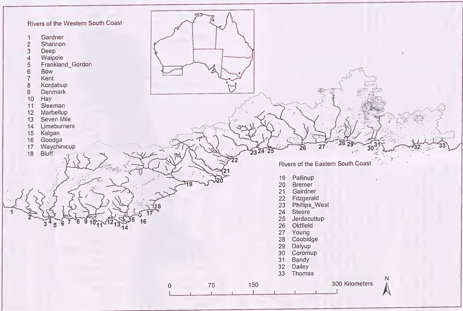
Figure 1. Map of South Coast Region showing location of waterways sampled.
